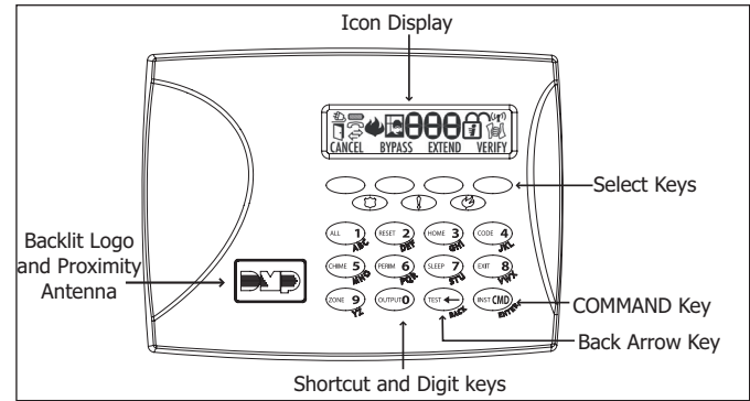
Thinline™ Series Icon Keypad
